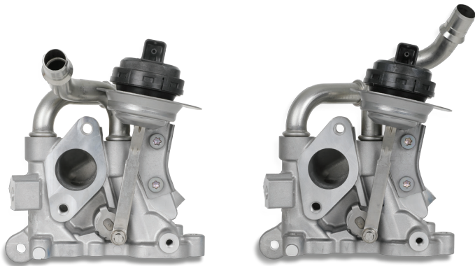
EGR bypass valve
